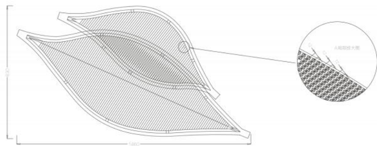
仰视图 / Upward View
